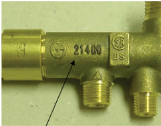
Fig. 1 Part #73416 Casting #21400
